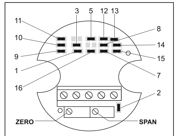
Bulk Head Temperature Transmitter
